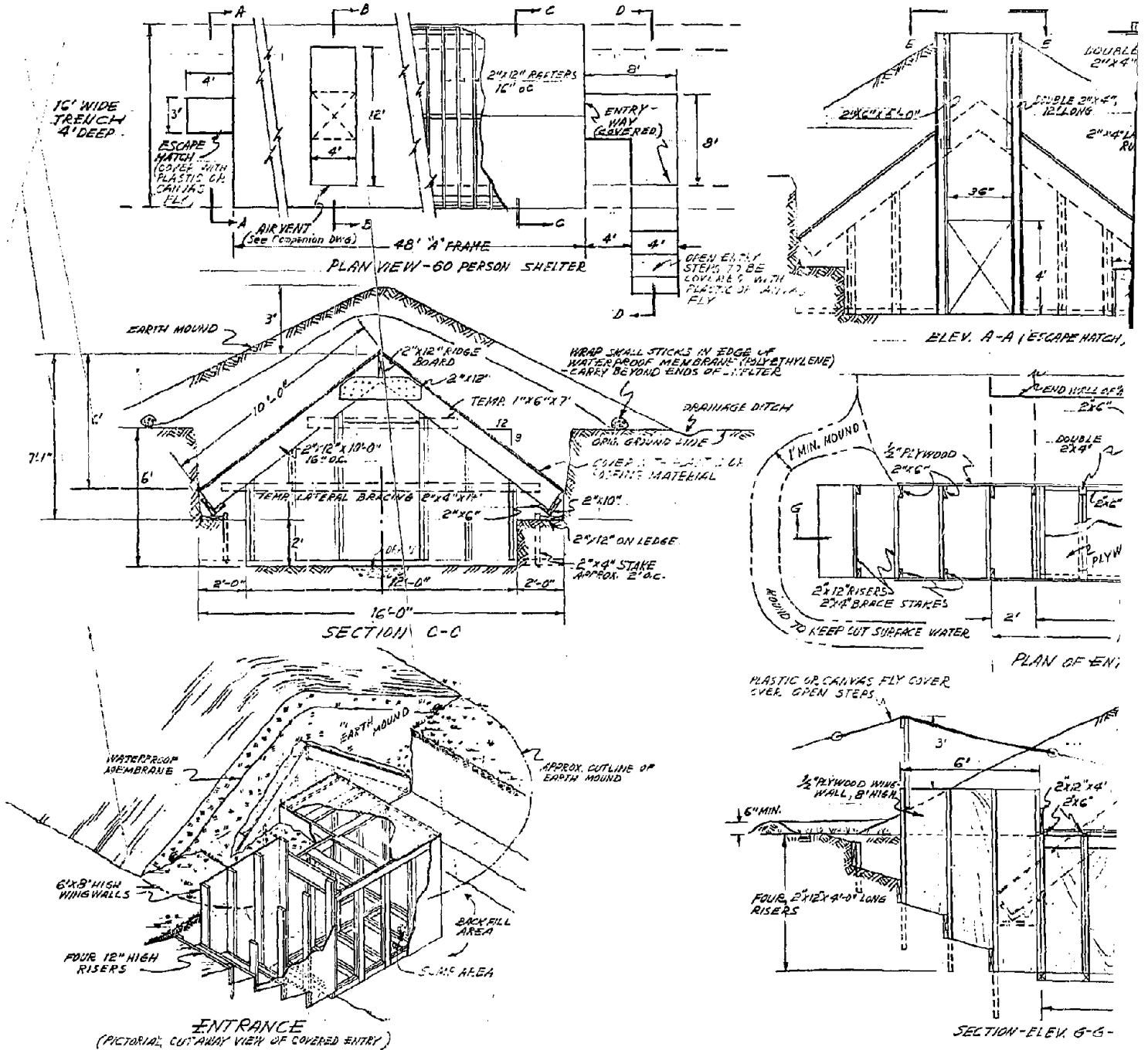
Fig. A-10.1. "A"-Frame Expedient Shelter, Plans and Elevation.
